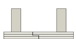
Variant 26 Shiplap edge (half thickness/50 mm) Total height: 160–490 mm
