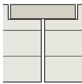
Variant 13 Standard rabbeting 23/51 mm alternatively 28/51 mm Thickness: 60–280 mm
