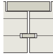
Variant 15 9 x 30 mm separate tongue standard rabbeting 23/51 mm alternatively 28/51 mm Thickness: 100–280 mm
