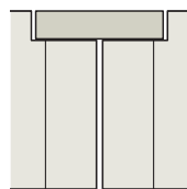
Variant 3 Standard rabbeting 23/51 mm alternatively 28/51 mm
