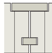
Variant 5 19 x 38 mm separate tongue standard rabbeting 23/51 mm alternatively 28/51 mm
