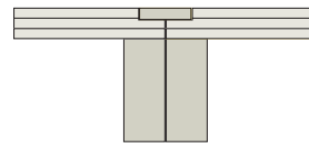
Variant 43 Standard rabbeting 23/51 mm alternatively 28/51 mm Total height: 160–490 mm
