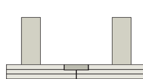
Variant 23 Standard rabbeting 23/51 mm alternatively 28/51 mm Total height: 160–490 mm
