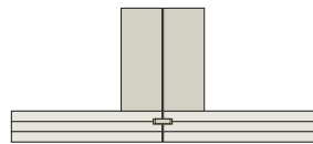
Variant 42 9 x 30 mm separate tongue Total height: 160–490 mm
