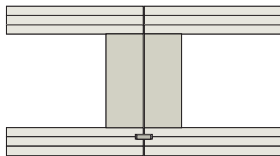
Variant 32 9 x 30 mm separate tongue CLT BOX – CEILING, height: 220–480 mm CLT BOX – CEILING FS, height: 260–490 mm
