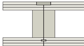
Variant 35 9 x 30 mm separate tongue Standard rabbeting 23/51 mm alternatively 28/51 mm CLT BOX – CEILING, height: 220–480 mm CLT BOX – CEILING FS, height: 260–490 mm
