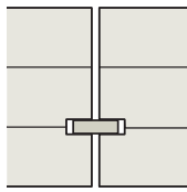
Variant 12 9 x 30 mm separate tongue Thickness: 60–280 mm
