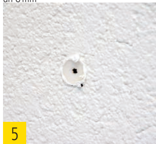
5 Remove any excess FDM WALL between plaster and spiral anchor.
