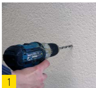
1 Pre-drilling of the rendered wood fiber insulation board by means of an 8 mm
