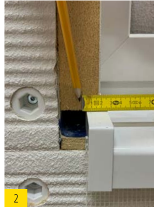
2 Scribe 20 mm and mark what is to be cut out.
