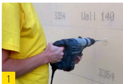
Pre-drilling by means of an impact drill.
