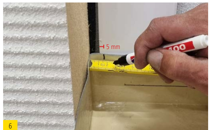
6 Mark the lip 5 mm inside the side edge of the window.
