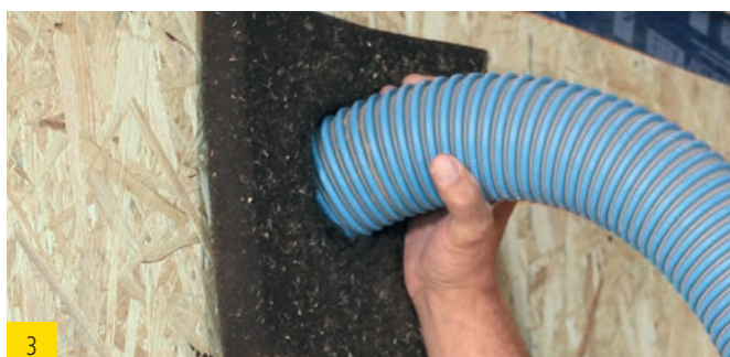
3 Inject air injected wood fiber insulation
